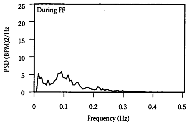
FIGURE 11 Mean power spectra before (baseline) and during the FF intervention (left) for the workplace study.
