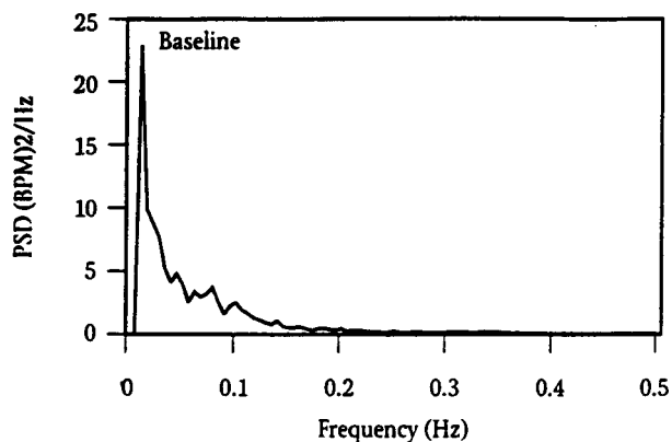
FIGURE 11 Mean power spectra before (baseline) and during the FF intervention (left) for the workplace study.
