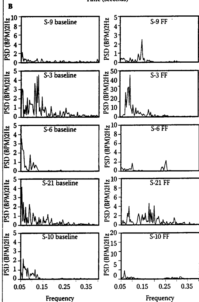
FIGURE 9 A representative sample of the workplace study A, real-time HRV data for subjects 9, 3, 6, 21, and 10 before and after the Freeze-Frame intervention. B, corresponding HRV power spectra. Note the ordinate scale changes.
