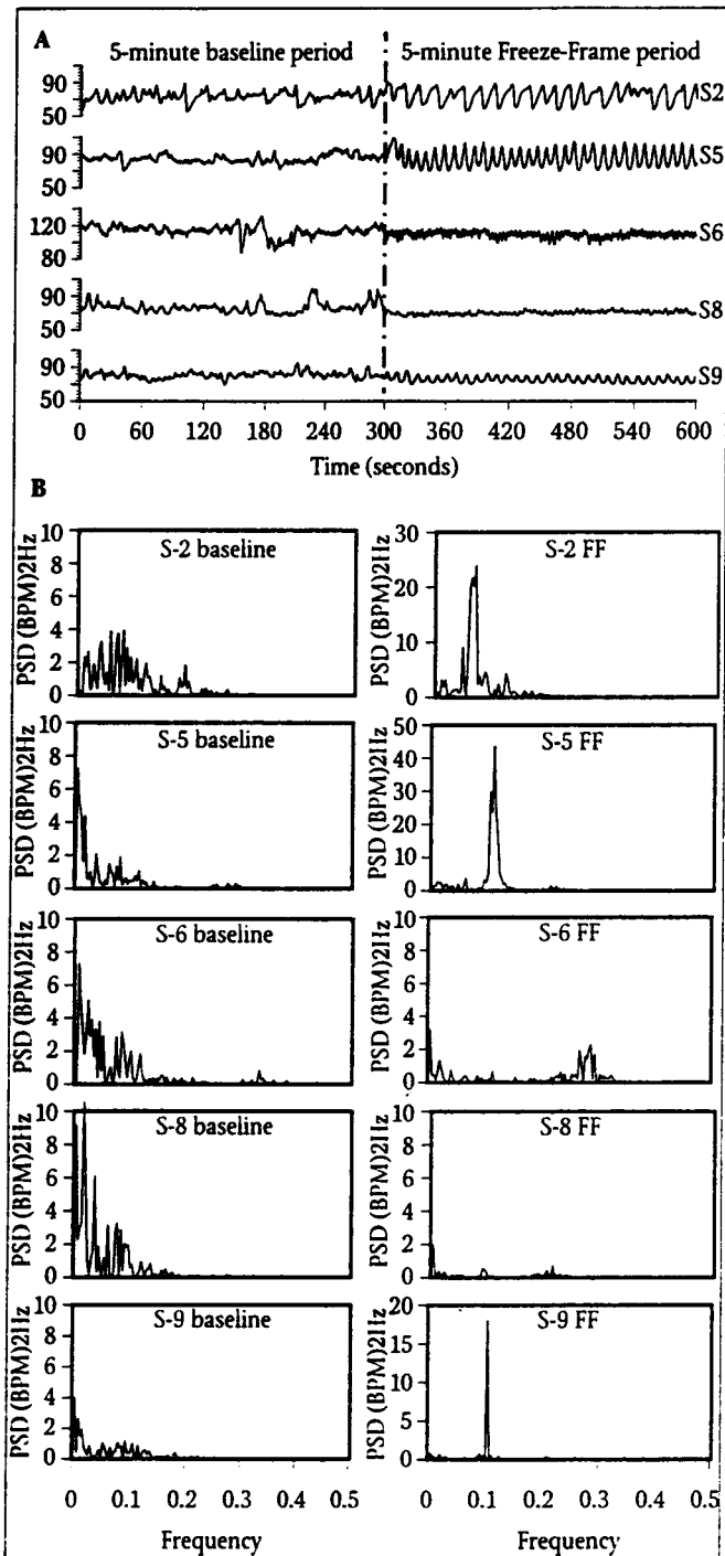
FIGURE 6 A representative sample from the laboratory study. A, real-time HRV data for subjects 2, 5, 6, 8, and 9 before and after the Freeze-Frame intervention. B, corresponding HRV power spectra. Note the large difference in ordinate scales for subject 5.
