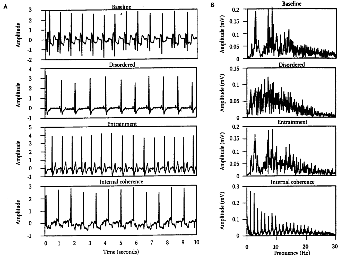
FIGURE 4 A, ECG recordings of heart function mode for subjects in four feeling states. From top to bottom, these are baseline, frustration, appreciation and amplified peace. B, Corresponding amplitude spectra for the ECG associated with each feeling state.
