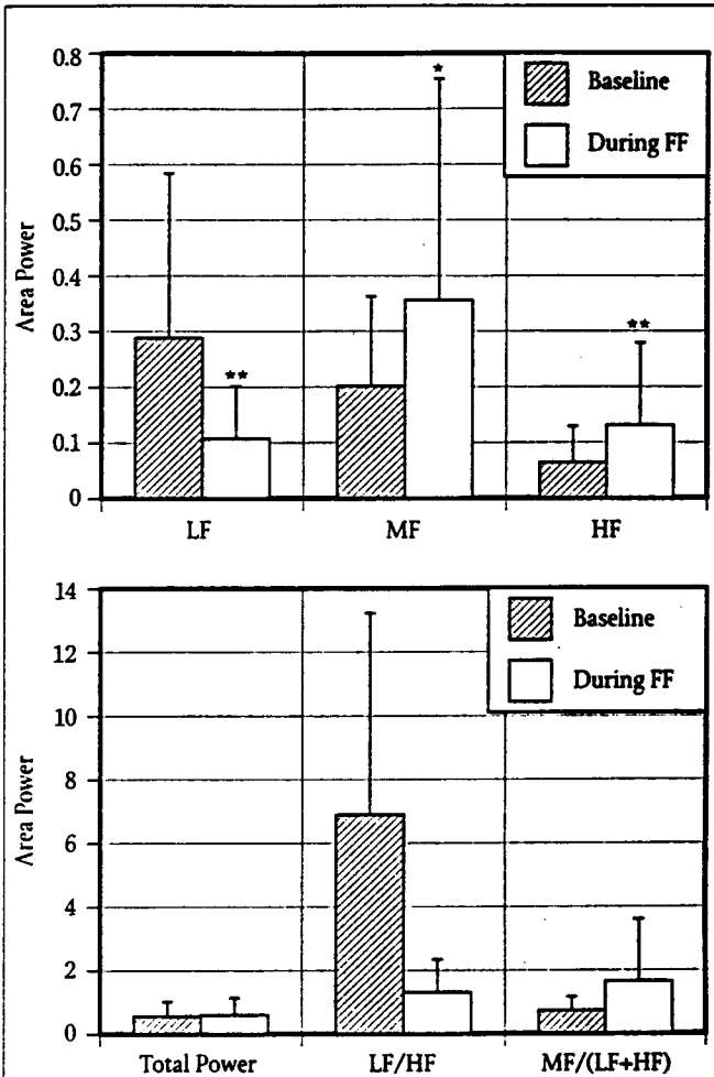
FIGURE 10 Mean integral power of group in LF, MF, HF, LF/HF and MF/(LF+HF) and total power across all frequency bands for the workplace study. * P < .05 ; ** P < .01 .
